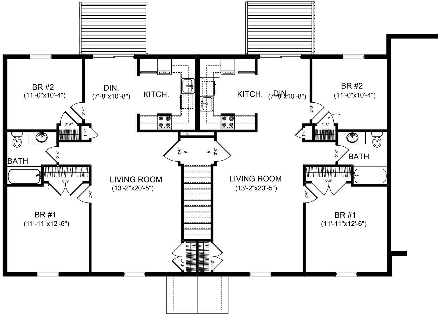
TYPICAL SECOND FLOOR UNIT
