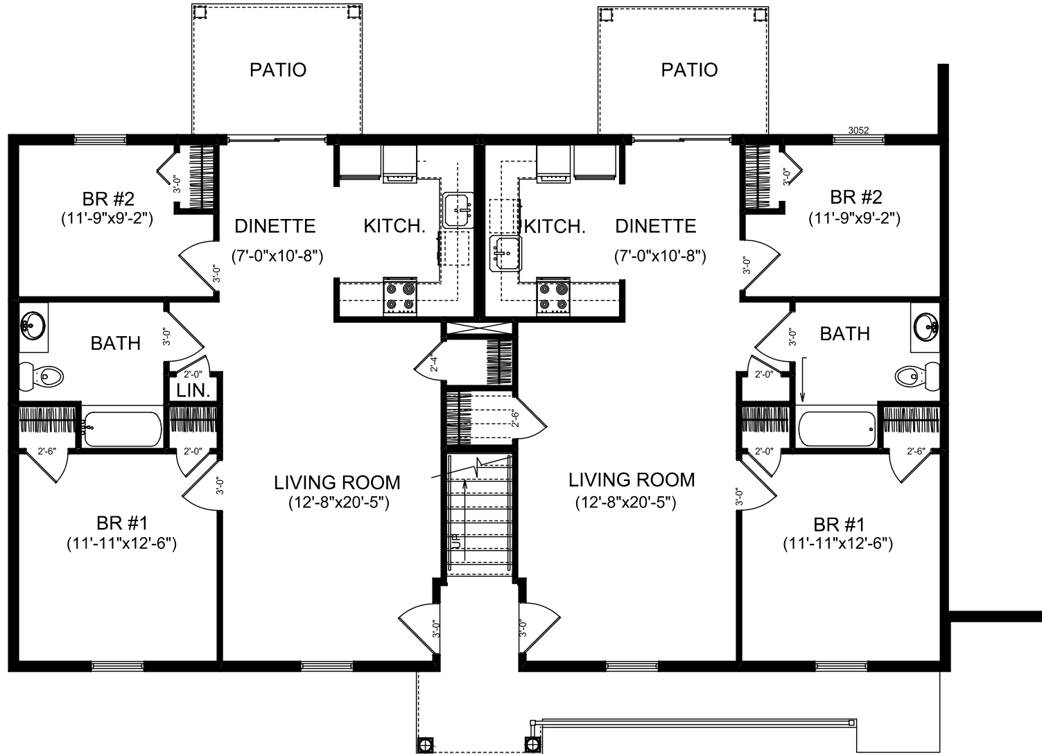
TYPICAL FIRST FLOOR UNITS
